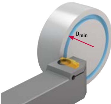
Right-hand tool G4521...R Shank design 90°
